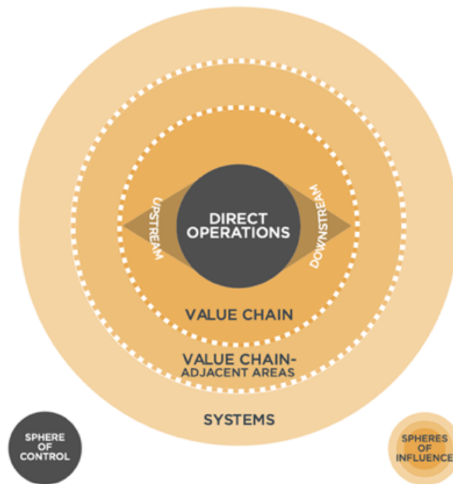
Figure 6. SBTN Spheres of Control Diagram 9
