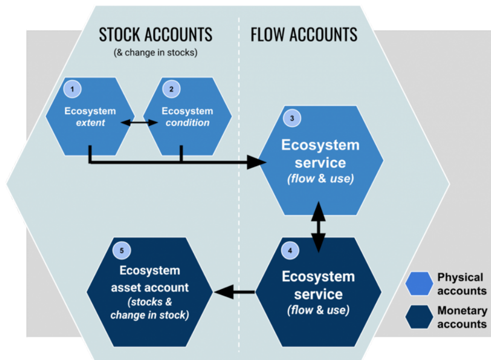
Figure 3. The general ecosystem accounting framework of the UN SEEA EA 5 . Accounting for Nature ® Certified Environmental Accounts can be used as Stock Accounts under the UN SEEA Ecosystem Accounts. Accounting for Nature Accredited Methodologies can be used to comply with the UN SEEA EA Ecosystem Condition Typology.
