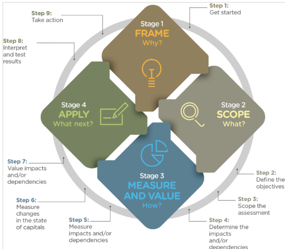
Figure 7. Overview of the Natural Capital Protocol Process 10
