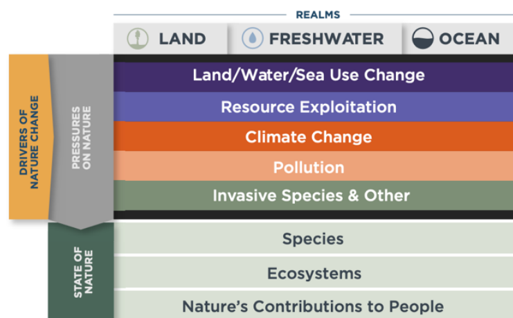
Figure 5. Overview of SBTN Target Categories 8 .
