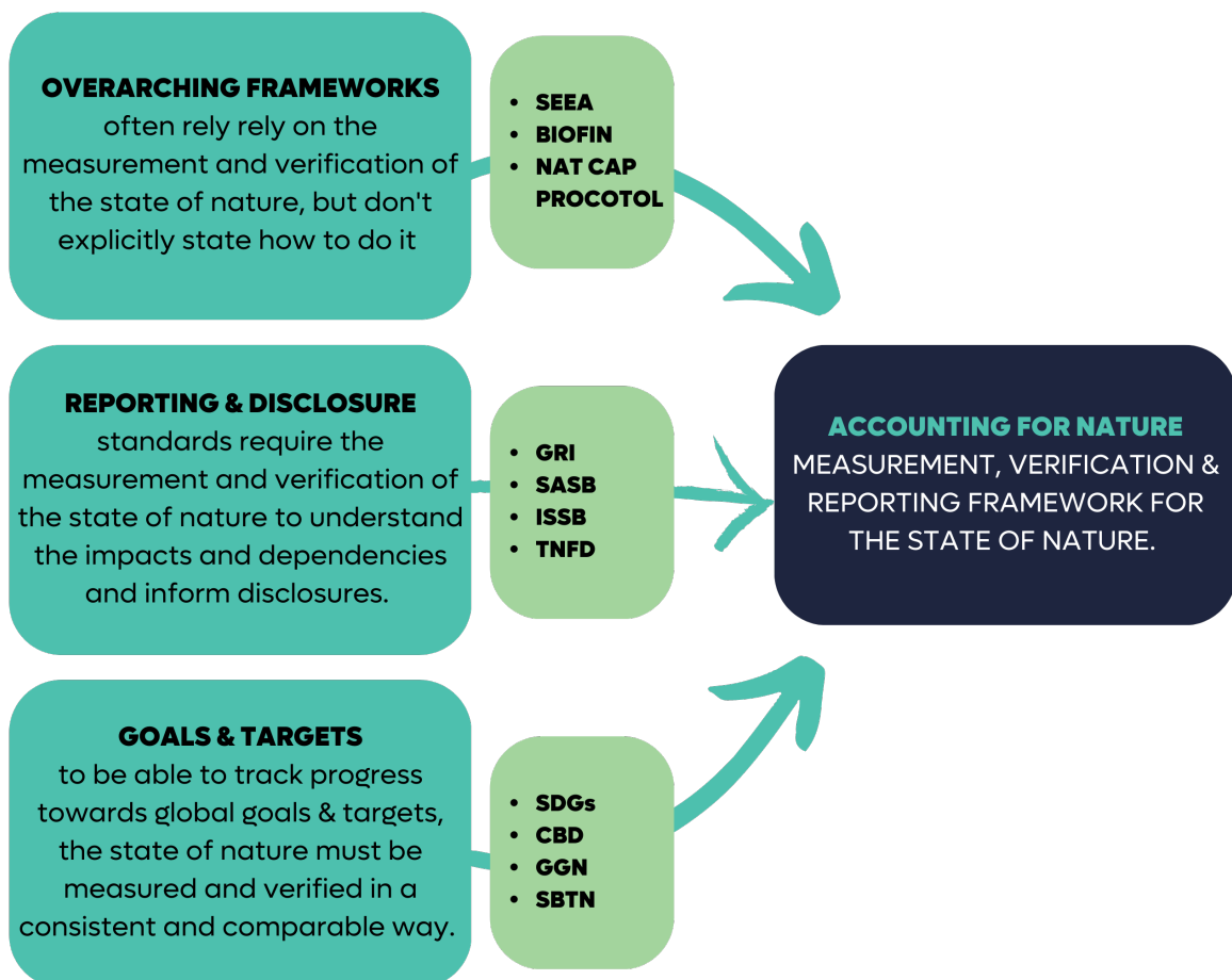
Figure 1. Overview of Accounting for Nature's® position among Global Frameworks.
